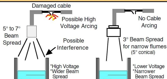
Competitor Designs US70TC Sensor Design
